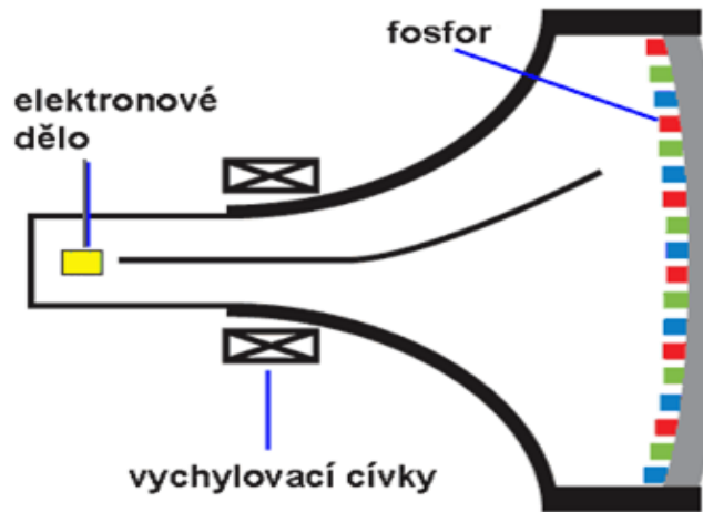
CRT
